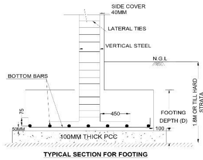
TYPICAL SECTION FOR FOOTING
