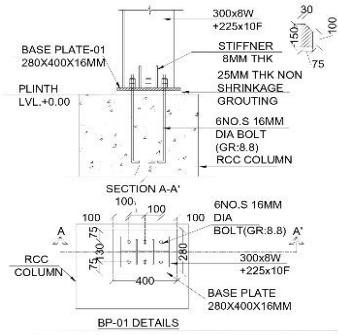
BP-01 DETAILS
