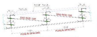
TYPICAL SAG ROD DETAIL @ ROOF
