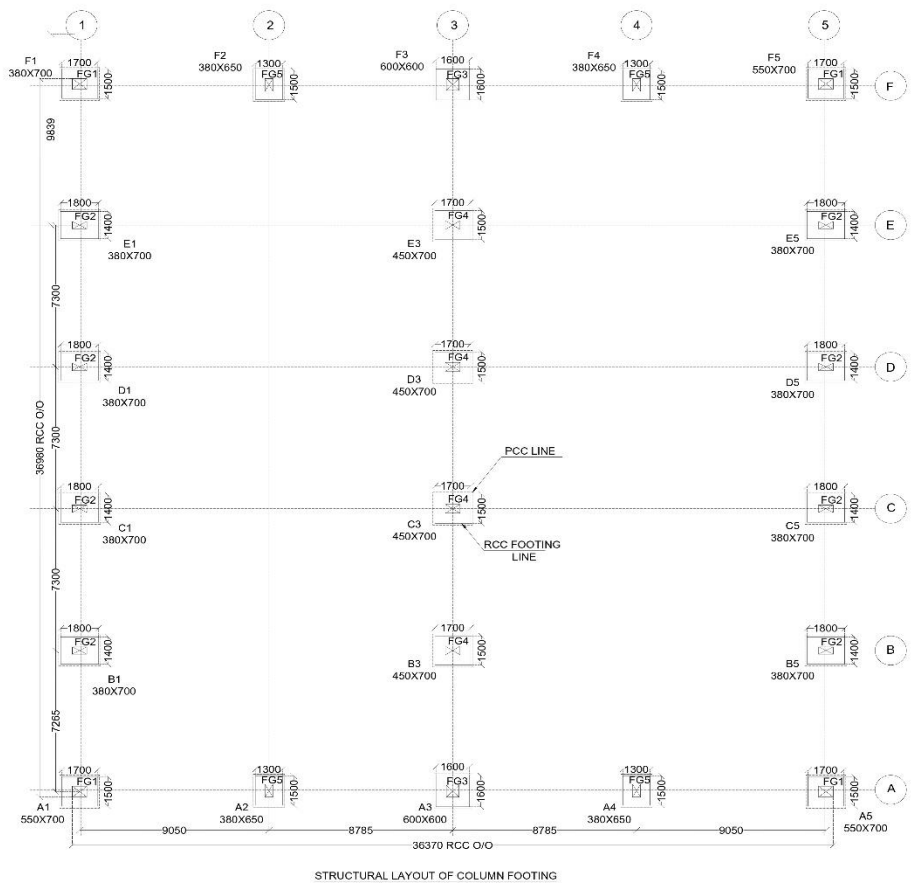
STRUCTURAL LAYOUT OF COLUMN FOOTING
