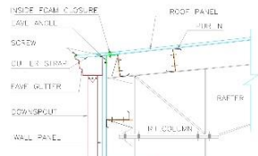
EAVE GUTTER DETAIL
