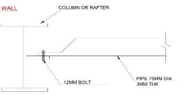
TYP. DETAILS FOR BRACING RAFTER/COLUMN CONNECTION
