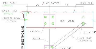
GABLE TRIM DETAIL
