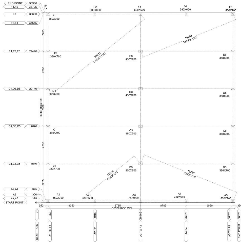
CENTER LINE PLAN
