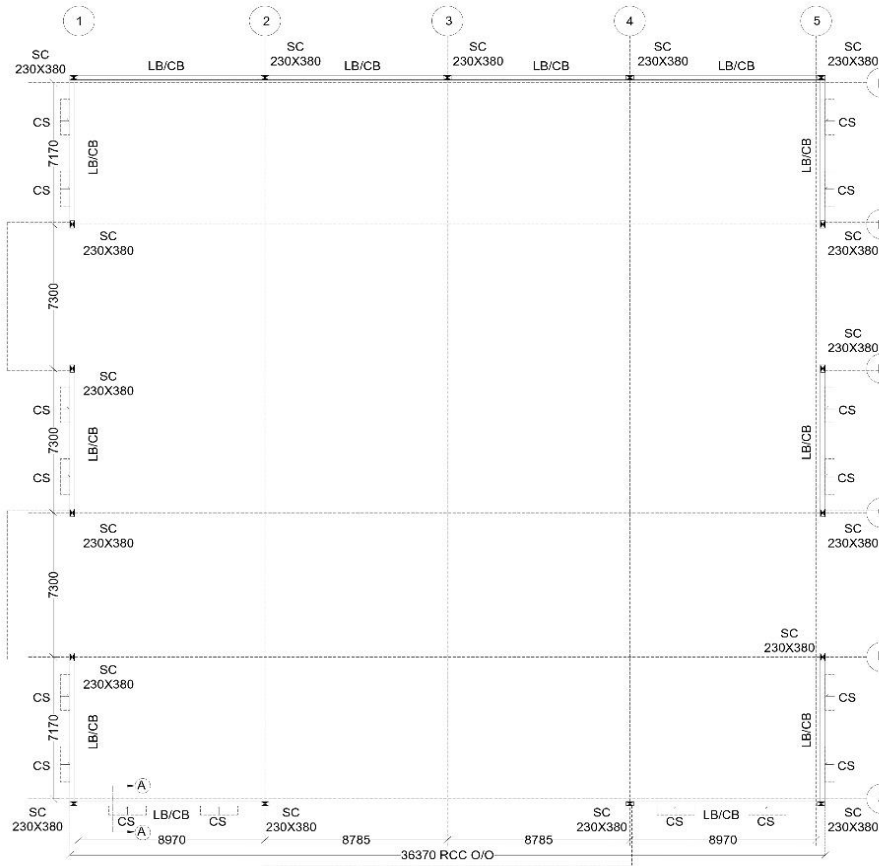
STRUCTURAL LAYOUT OF LINTEL BEAM RESTING OVER BRICKWORK
