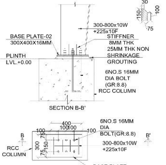
BP-02 DETAILS
