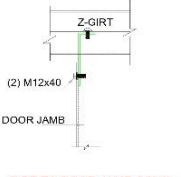
Z-GIRT TO DOOR JAMB CONN.
