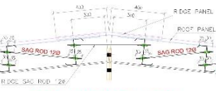
TYPICAL SAG ROD DETAIL @ RIDGE
