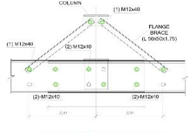
GIRT LAP DETAIL (SHORT LAP)
