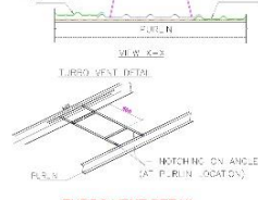
TURBO VENT DETAIL (AS & WHERE REQUIRED)
