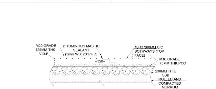
TYPICAL TRIMIX DETAILS
