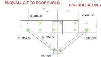
PURLIN CONN. AT INTERIOR RAFTER (SHORT LAP)
