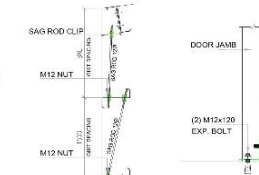
SAG ROD DETAIL @ WALL FOR LOW BAY
