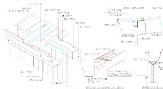
EAVE GUTTER ARRANGEMENT FOR ROOF PANEL AND DOWNSPOUT ARRANGEMENT WITH WALL PANEL
