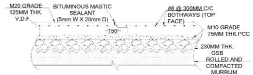
TYPICAL TRIMIX DETAILS
