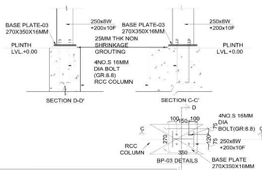
BP-03 DETAILS
