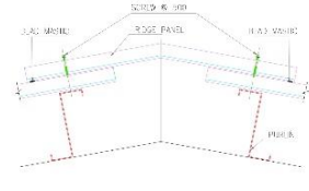
RIDGE PANEL DETAIL
