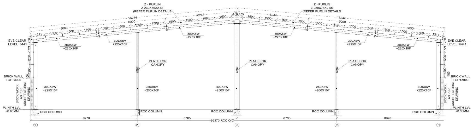
GABLE FRAME @ GL A
