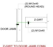
Z-GIRT TO DOOR JAMB CONN. DETAIL
