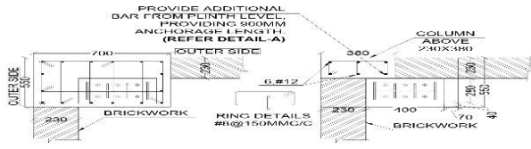
BOLT PLATE DETAILS WITH R/F OF COLUMN A1, A5, F1, F5 (REFER PEB DETAIL: BP-01)
