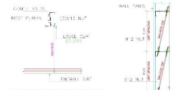
TYP. DETAIL OF SAG ROD FOR ENDWALL GIRT TO ROOF PURLIN
